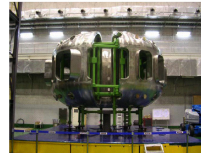
Fig. 13 Vacuum vessel after site welding
