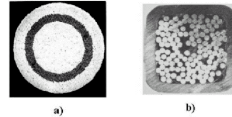
FIG. 3. Cross-section of a) the superconducting strand (0.86 mm diameter) and b) the CICC used for superconducting magnets of SST-1.
