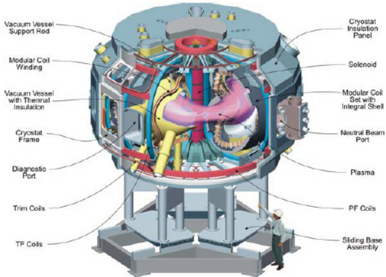
Figure 1. Details of the National Compact Stellarator Experiment
