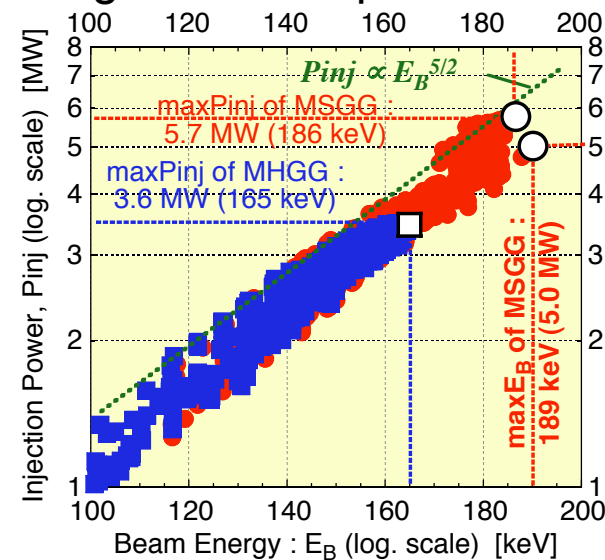
Progress of NB power in LHD
