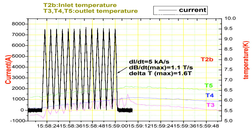
AC losses test
