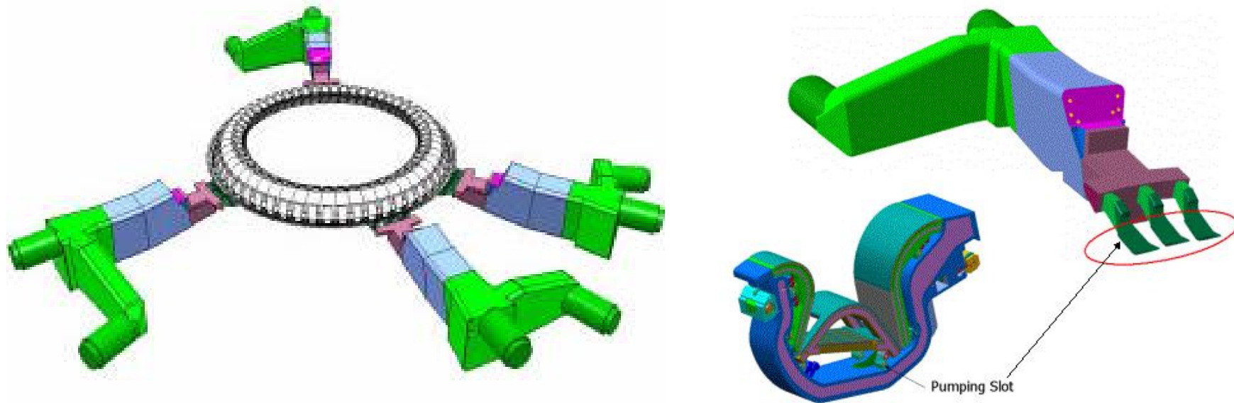
FIG. 1. Left: 3D view of the ITER exhaust gas pumping port geometry showing the connection to the branched and direct cryopumps. Right: Detailed view of the individual divertor cassette and the three fingered connection to the duct, highlighting the pumping slot cross-section.
