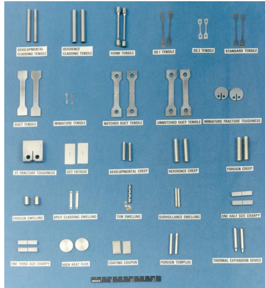
Example of SSTT specimens for IFMIF
