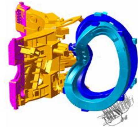
Modular coils mounted onto the coil support ring.
