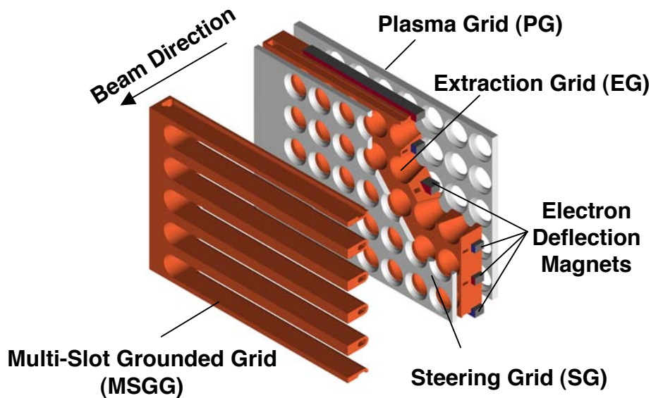
Accelerator structure in LHD N-NBI
