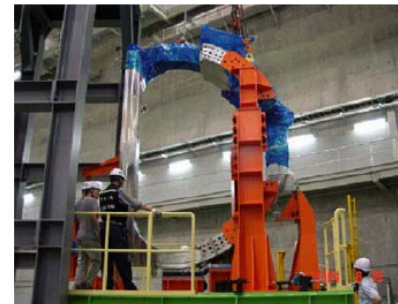
Fig. 8 Loading the TF00 magnet on the lower TF-transporter
