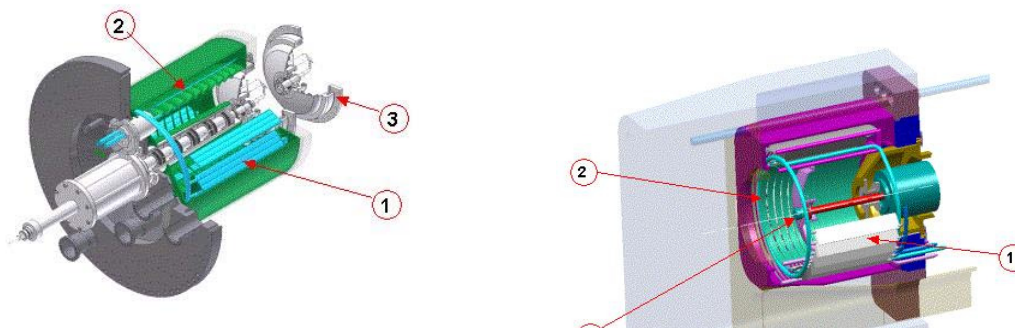
FIG. 2. Comparison of the TIMO model pump (left) and the ITER 1:1 torus exhaust cryopump (right) showing the pumping panels (1), baffles (2) and the inlet valve (3).
