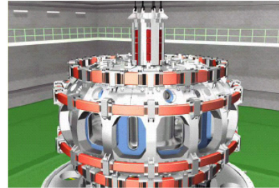
Fig. 3 Schematic drawing - assembling the central solenoid coils
