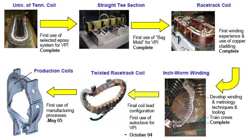
Figure 7. NCSX Modular Coil Winding Manufacturing R&D Studies
