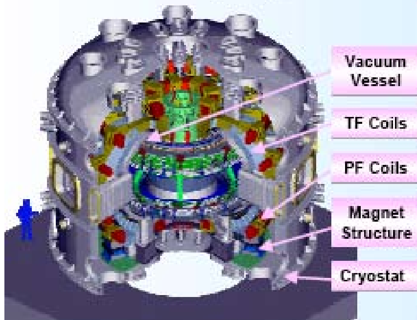
KSTAR Device & Major Components
