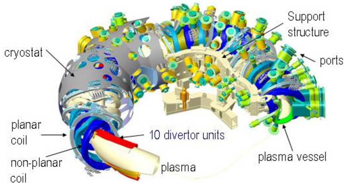
Components of Wendelstein 7-X.
