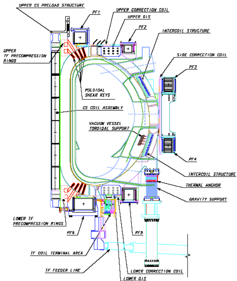
Cross-section of ITER magnets
