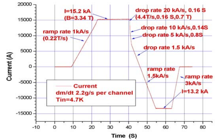
Current charge/discharge
