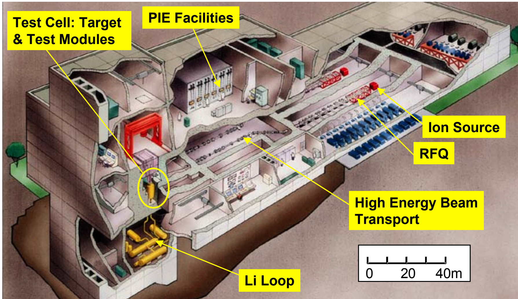
The International Fusion Materials Irradiation Facility (IFMIF)
