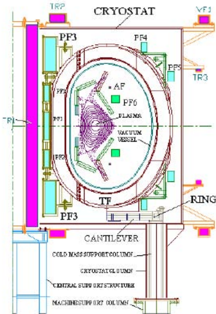
A cross-section of SST-1 Tokamak
