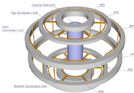
Saddle coils
