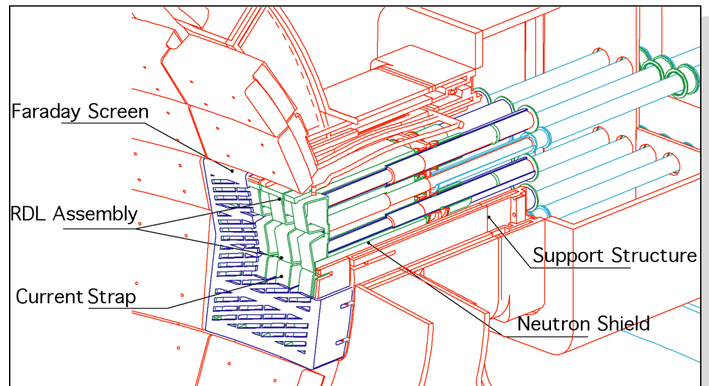
ITER ICRF Launcher (Baseline Design)
