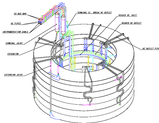
Central Solenoid
