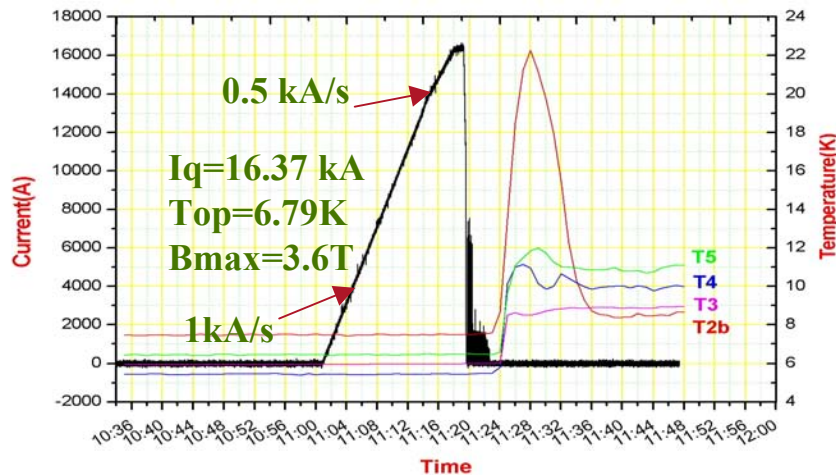
Quench current test
