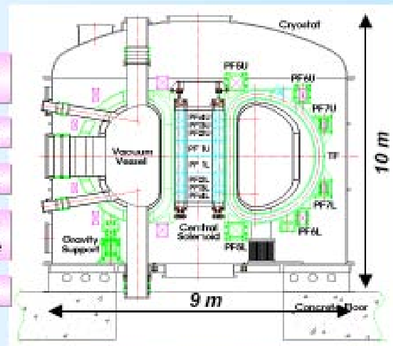
Elevation View of KSTAR
