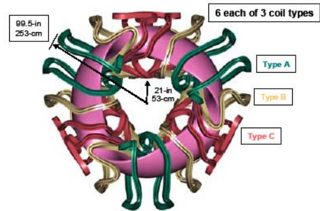
Figure 4. The NCSX plasma and modular coil system.
