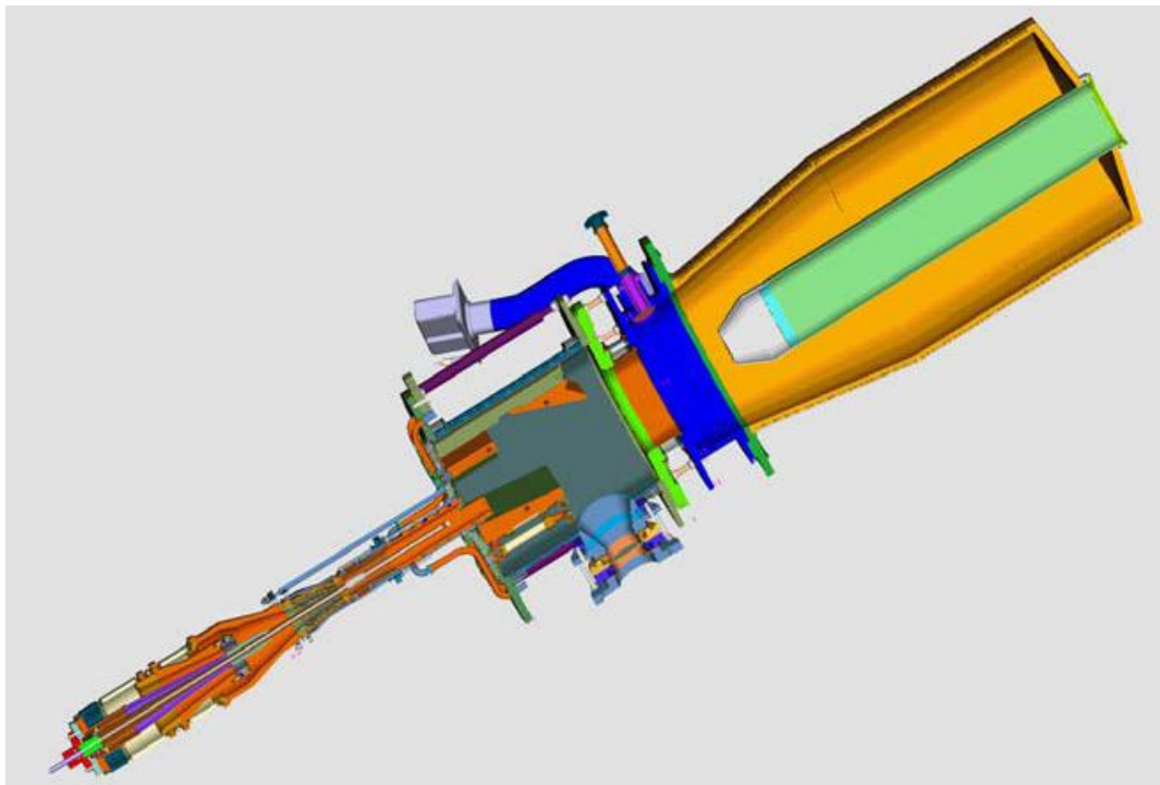
Fig. 1. Cut of the integrated 170 GHz, 2 MW, CW coaxial cavity
