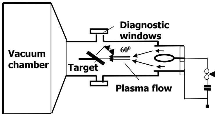
The diagram of QSPA facility
